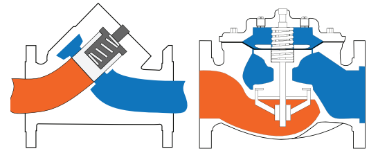
Piston Valve
